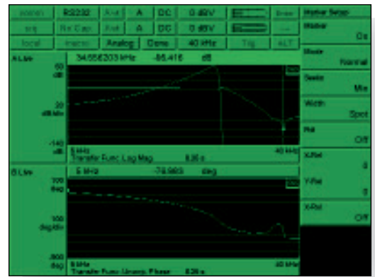
Swept-sine Bode plot of lowpass filter response. Top display shows magnitude with an expanded view of the passband response, while bottom display shows the phase response.
